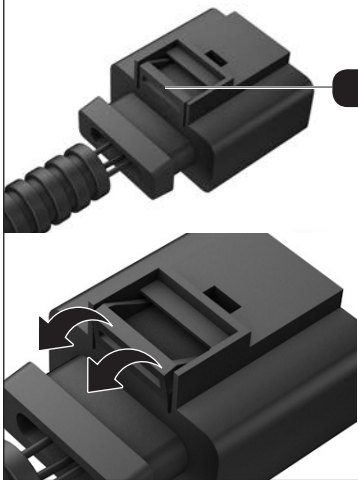
Locking clip
